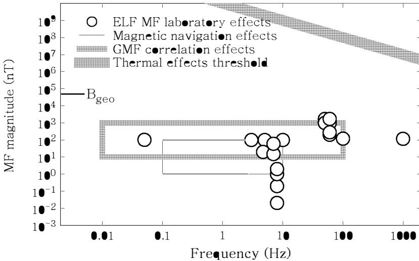
Figure 12. Frequency-magnitude diagram of the observable biological effects of superweak MFs. The frequency range for magnetic navigation is conditional.
