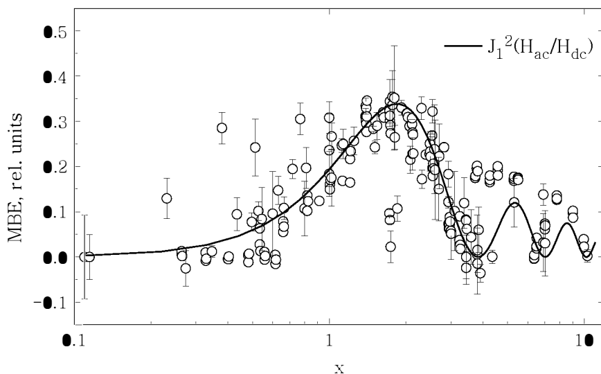
Figure 14. Theoretical amplitude spectrum (solid curve) calculated for ion-protein complexes; MBEs (points) in parallel ac/dc MFs as functions of x \sim H_{ac}/H_{dc} . Adapted from the data analyzed in (Binhi, 2002).
