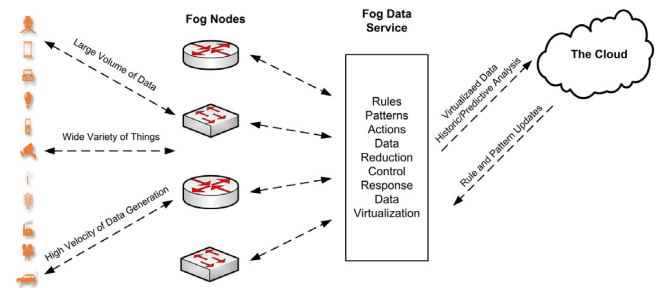
Fig. 4. Fog data services coordinate the movement of data from fog to cloud [33].
