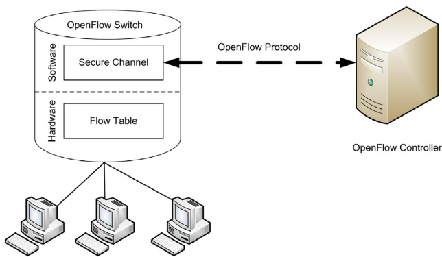
Fig. 2. OpenFlow protocol [26].
