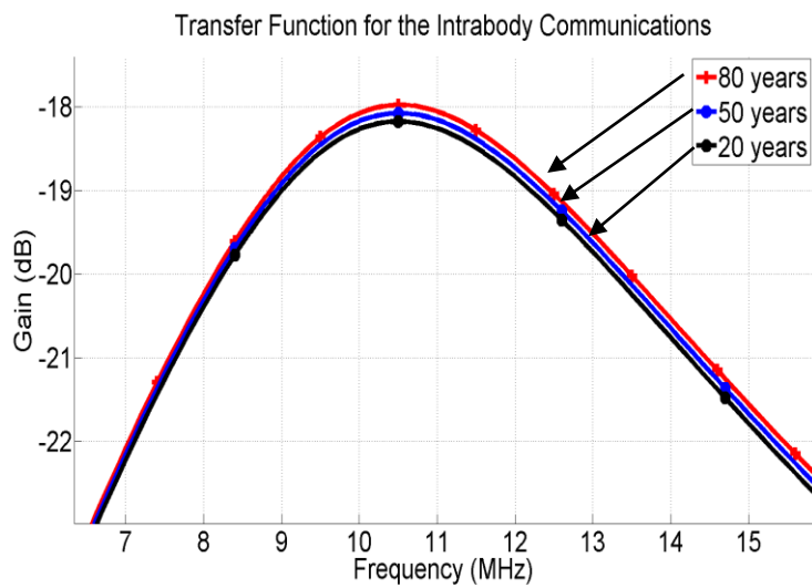
Figure. 3.16: Simulation results, showing the channel sensitivity to the individual's age, where gain is plotted for three different age groups; 20, 50 and 80 years old.
